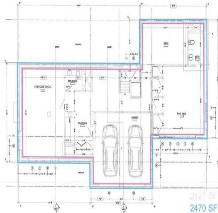
6 PINTAIL - BASEMENT FLOOR PLAN - NTS
