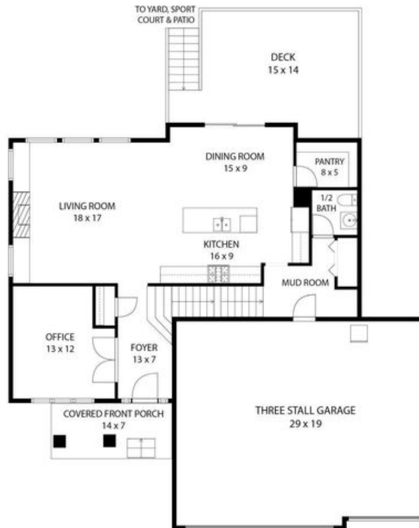
MAIN LEVEL FLOOR PLAN 20164 HARVEST DRIVE, LAKEVILLE
